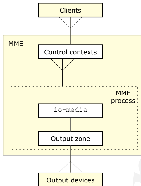
Client, control context, MME process, io-media , output zone and output device relationships.
